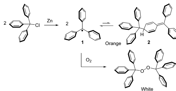
Fig. 2 Triphenylmethyl radical and its derivatives.
