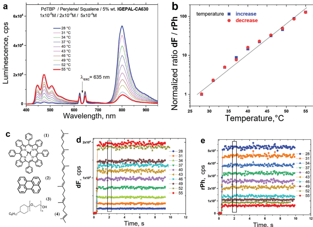
Fig. 15 (a) Dependence of the luminescence spectra of the micellar TTA–UC system. Material composition is as follows, PdTBP/peryene/squalene/IGEPAL-CA630 in an aquatic environment on the sample temperature. The concentrations of the active materials are as follows, 1 \times 10^{-5} \text{ M} / 2 \times 10^{-4} \text{ M} / 5 \times 10^{-4} \text{ M} / 5 \text{ wt\%} in water; (b) temperature calibration curve: ratiometric response, representing the normalized ratio of the delayed upconverted fluorescence and residual sensitizer phosphorescence as function of the sample temperature; (c) structure of the active materials, as follows: (1) meso -tetraphenyl-tetrabenzoporphine Palladium (PdTBP); (2) dibenz[ de,k ]anthracene (peryene); (3) octylphenyl-polyethylene glycol (IGEPAL-CA630); (4) 2,6,10,15,19,23-Hexamethyl-2,6,10,14,18,22-tetracosahexaene (squalene); (d) temporal dependence of the delayed fluorescence for different sample temperatures; (e) temporal dependence of the residual phosphorescence for different sample temperatures. Conditions: the excitation intensity is constant, 100 \text{ mW} \times \text{cm}^{-2} for all measurements; cw – diode laser \lambda = 635 \text{ nm} ; excitation spot diameter – 1000 \mu\text{m} ; sample thickness – 400 \mu\text{m} ; an oxygen-free environment (the samples are prepared and sealed in nitrogen-filled glove-box, 2 ppm \text{O}_2 residual concentration).
