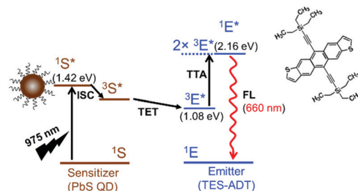
Fig. 1 Energy level diagram of the PbS QD:TES-ADT upconversion system. The chemical structure is that of TES-ADT.
