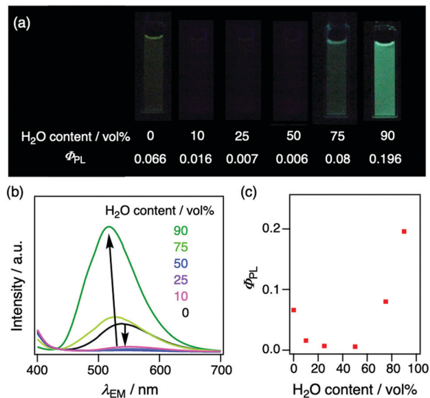
Fig. 5 (a) Photographs taken under blacklight ( \lambda_{\text{EX}} = 365 \text{ nm} ), (b) PL spectra, and (c) plots of absolute \phi_{\text{PL}} against H 2 O content (vol%) in THF solution of 2Cz2SB ( 2 \times 10^{-5} \text{ M} ).
