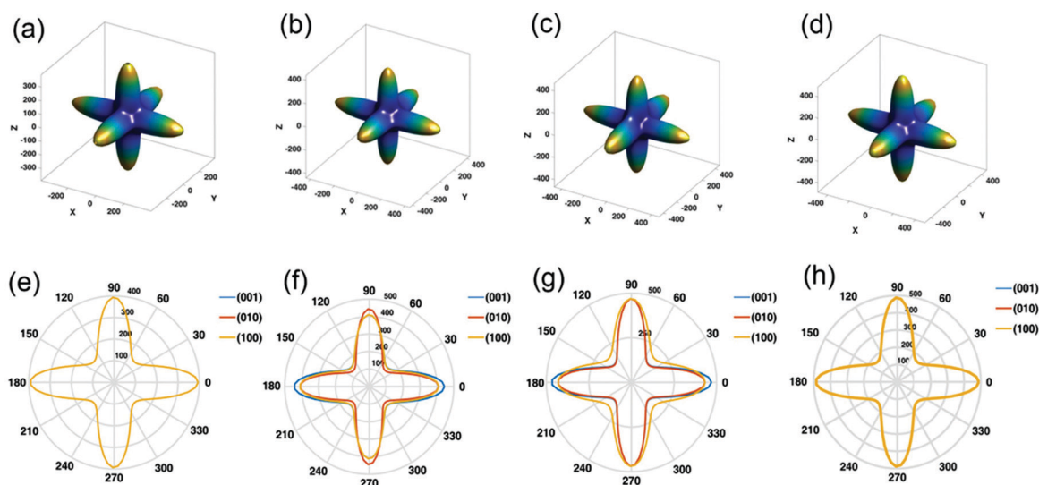
Fig. 8 3D Young's modulus: (a) CsPbI 3 , (b) CsPbI 2 Br, (c) CsPbI 2 Br 2 , and (d) CsPbBr 3 . 2D Young's modulus: (e) CsPbI 3 , (f) CsPbI 2 Br, (g) CsPbI 2 Br 2 , and (h) CsPbBr 3 . Reproduced with permission from ref. 128. Copyright©2020, Wiley Online Library.
