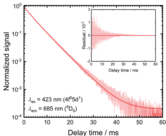
Fig. 2 The photoluminescence decay curve recorded upon monitoring the ^5D_0 \rightarrow ^7F_0 transition at 685 nm ( \lambda_{ex} = 423 \text{ nm} ) at room temperature. The solid red line indicates a single exponential fit and the inset depicts the respective residual plot.
