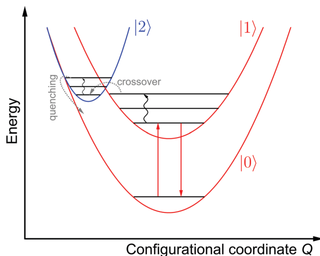
Fig. 3 Schematic overview of the different processes determining the performance of a luminescent crossover thermometer such as Sm^{2+} . Curvy arrows indicate (multi-)phonon absorption transitions. Note that the excited state |2\rangle has been depicted at lower configurational coordinates to match the theoretical and experimental findings for low excited 4f^{n-1} 5d^1 states of lanthanoid ions (see also text).
