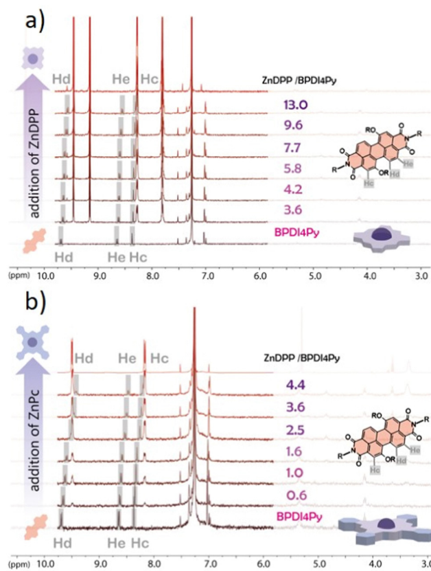
Fig. 5 (a) 1 H NMR spectra in CDCl 3 of a titration of BPD14Py solution (0.5 mL, 0.055 mM) with increasing amounts of ZnDPP (400 μL, 13 mM) in CDCl 3 . (b) 1 H NMR spectra in CDCl 3 of a titration of BPD14Py solution (0.5 mL, 0.055 mM) with increasing amounts of ZnPc (180 μL, 0.13 mM) in CDCl 3 .
