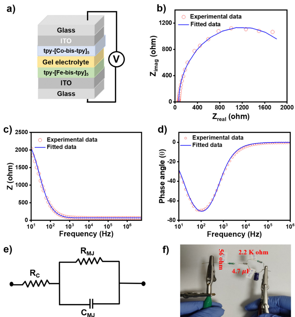
Fig. 7 (a) A schematic description of a molecular junction composed of ITO/ \text{tpy} -[ \text{Fe}(\text{bis-tpy})_5 ]/gel electrolyte/[ \text{Co}(\text{bis-tpy})_5 ]- \text{tpy} /ITO. (b) The Nyquist plot of the junction. (c and d) Bodes plot at varying frequencies. (e) The Randles equivalent circuit and (f) a real circuit for the experimental validation of the fitted model.
