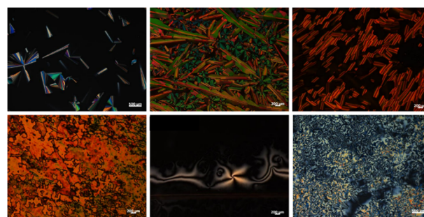
Fig. 4 Selected POM textures of some representative \pi -bridged dimers. Top row: \text{Tp}^6\beta - \text{Th}_2\text{Tp}^6 (100 °C, Col hex ), \text{Tp}^6\text{Fu}_2\text{Tp}^6 (228 °C, Col rec ), and \text{Tp}^6\text{Tt}_2\text{Tp}^6 (178 °C, Col hex ); bottom row: N Col of \text{Tp}^8\text{Th}_2\text{Tp}^8 (195 °C), \text{Tp}^6\text{Ph}_2\text{Tp}^6 (174 °C), and \text{Tp}^8\text{Ph}_2\text{Tp}^8 (165 °C). Additional textures can be found in Fig. S57 (ESI † ).
