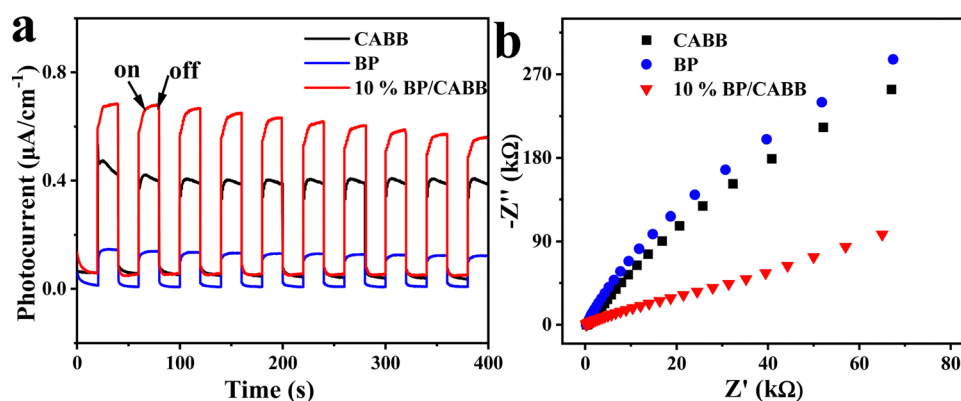
Fig. 7 (a) Chopped light amperometric I-t curves and (b) EIS Nyquist plots of CABB, BP and the 10% BP/CABB composite.
