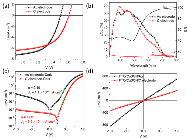
Fig. 3 (a) Light J-V curves and (b) external quantum efficiency of champion solar cells with Au and C electrodes, along with the reflectance spectrum of Au and C electrodes. (c) Corresponding dark J-V curves, used for the calculation of the device ideality factor ( n ) and reverse saturation current density ( J_0 ). (d) Linear J-V curve for FTO/CuSCN/electrode devices.
