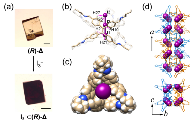
Fig. 5 Anion recognition in (R)- \Delta . (a) Photographs of single crystals of (R)- \Delta and \text{I}_3^- \subset (\text{R})-\Delta . Scale bars represent 200 \mu\text{m} . (b and c) Superstructure of \text{I}_3^- \subset (\text{R})-\Delta (b) in tubular and (c) space-filling representations exhibiting the encapsulation of \text{I}_3^- inside the cavity of (R)- \Delta by 18 [C-H...I] interactions. C, tan; N, blue; H, white; I, purple. (d) Side-on (top) and top (down) views of the double helical superstructure of \text{I}_3^- \subset (\text{R})-\Delta . Hydrogen atoms are omitted for clarity. One strand in the double helix is depicted in orange tubular representation and the other in blue, while \text{I}_3^- is represented in a space-filling form.
