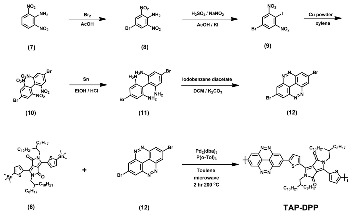
Scheme 2 Synthesis route of monomer (12) and TAP-DPP.
