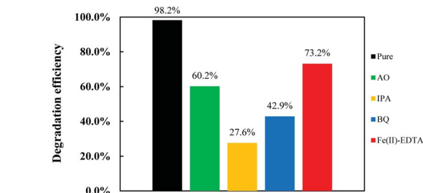
Fig. 10 Effect of radical scavengers on the POME degradation efficiency using the {001}- \text{TiO}_2/\text{Ti}_3\text{C}_2 aerogel composite.
