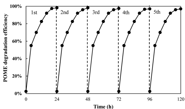
Fig. 7 Photostability test of the TiO 2 /Ti 3 C 2 MXene aerogel composite for POME degradation.
