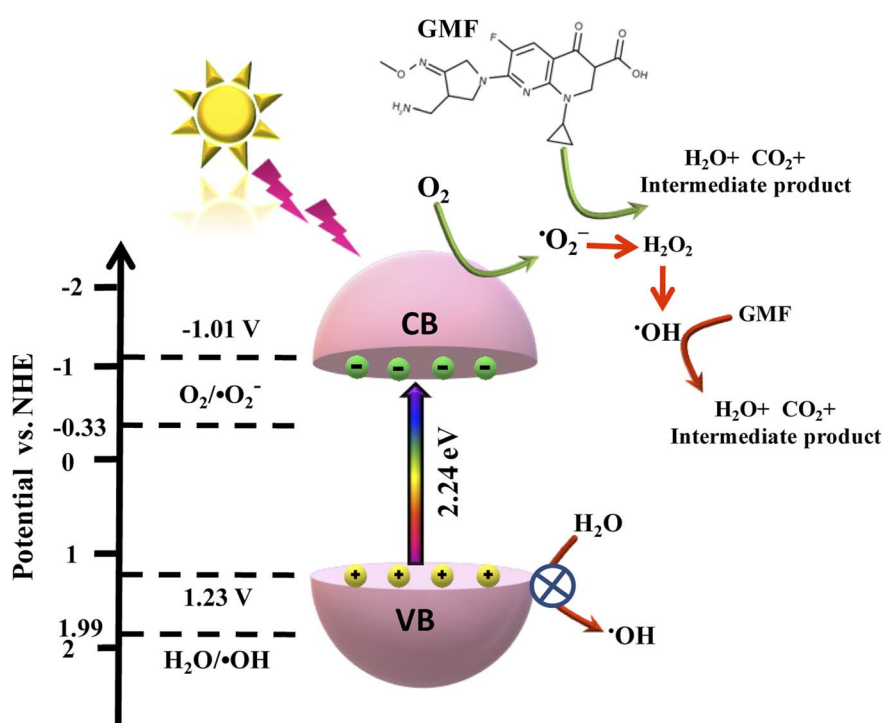
Scheme 3 Feasible mechanism for the degradation of GMF over \text{Cu}_{0.75}\text{In}_{0.25}\text{S} QDs via \cdot\text{O}_2^- and \cdot\text{OH} radical under 20 \text{ W} visible-LED lamp.
