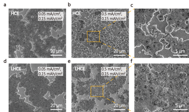
Fig. 4 Top-view SEM images of K deposition morphologies in (a–c) HCE and (d–f) LHCE with enlarged views (c and f) at a current density of (a and d) 0.05 \text{ mA cm}^{-2} and (b and e) 0.5 \text{ mA cm}^{-2} with a capacity of 0.15 \text{ mA h cm}^{-2} .
