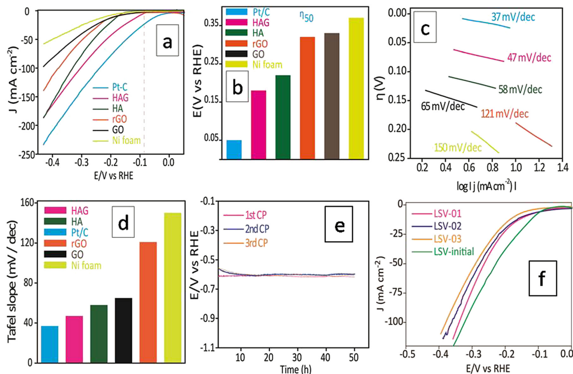
Fig. 7 HER electrocatalytic performance of HAG. (a) Polarograms of HAG, HA, rGO, GO, Pt-C, and Ni foam is taken at 2 mV s -1 without iR correction. (b) Bar diagram showing the \eta_{50} values of all materials. (c) Tafel slope comparison. (d) Bar diagram showing the Tafel slope values compared between the catalysts. (e) Chronoamperometric stability experiment and activity reproducibility test of HAG. (f) Polarograms recorded after each CP experiment.
