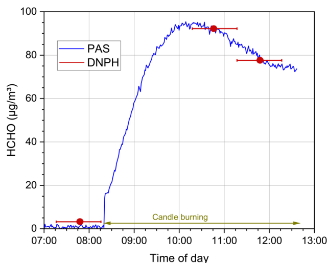
Fig. 9 Time course of the formaldehyde concentration when burning a candle in a 1 \text{m}^3 test chamber according to EN 16738 115 ( T = 23^\circ\text{C} , relative humidity = 50%, air exchange rate = 2 \text{ h}^{-1} , see also Salthammer et al. 116 for the detailed experimental conditions). The blue curve represents the online measurement with a photoacoustic device (Gasera One), the red dots are the concentrations determined from a 60 min sampling using the DNPH method, the red lines indicate the duration of the sampling.
