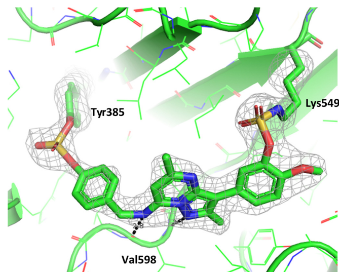
Fig. 13 Crystal structure of 11 engaged with Lys 549 and Tyr 385 in PI4KIIIβ and a corresponding F_o - F_c difference “omit” map contoured at 3\sigma (grey mesh) [PyMOL 47 generated figure] (PDB: 8Q6H). The compound is present in the ATP binding site and makes key H-bonding interactions with hinge residue Val 598 .
