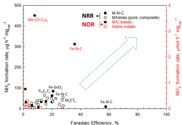
Fig. 5 Selection of representative electrocatalytic results in the nitrogen reaction and oxidation reactions (NRR and NOR, respectively): faradaic efficiency versus the rate of ammonia or nitrate formation at ambient conditions. The dashed arrow indicates the gap in the electrocatalytic results to meet requirements for industrial exploitability. M–N–C: nitrogen/metal-doped carbons.
