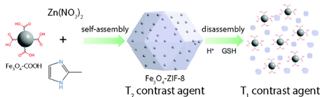
Fig. 17 T_1 - T_2 responsive Fe_3O_4@ZIF-8 nanosystem assembly and disassembly triggered by pH and glutathione (GSH). Adapted from ref. 132.
