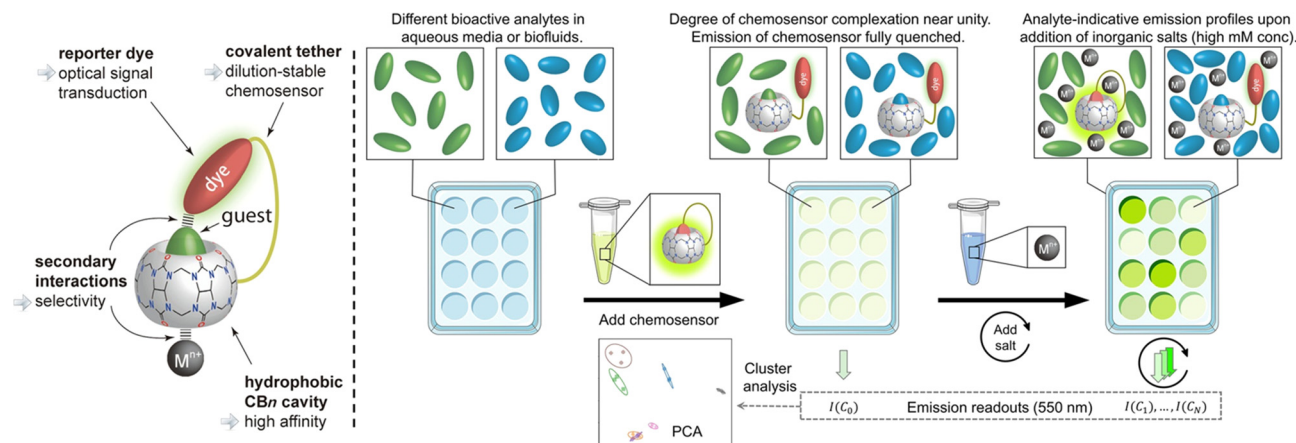
Fig. 30 Schematic representation of the unimolecular CB n -based chemosensor that undergoes salt-induced adaptation and that can be used for the distinction of bioorganic analyte in aqueous media and biofluids. Reproduced with permission from ref. 135. Copyright 2022 American Chemical Society.
