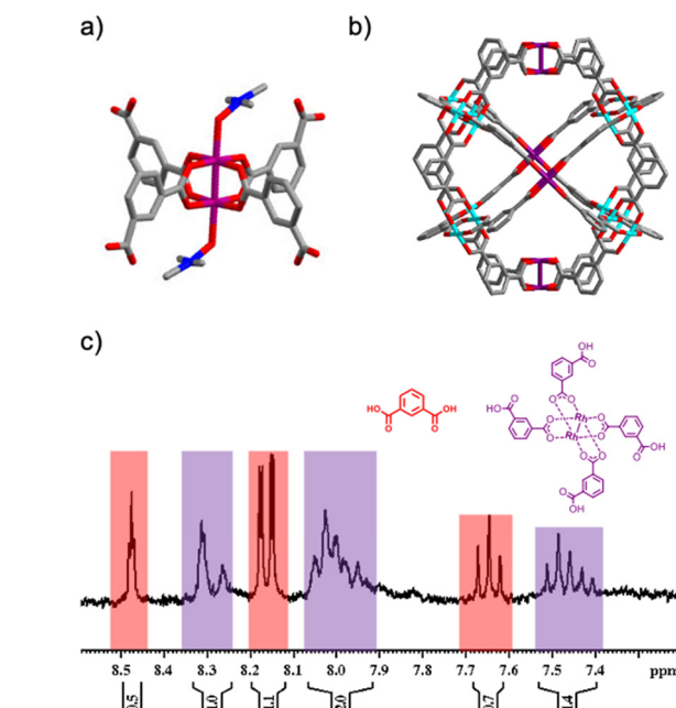
Fig. 2 (a and b) Crystal structures of (a) deprotected \text{Rh}_2(\text{bdc})_4 complex and (b) HET-MOP-1. (c) 1 H NMR spectrum (300 MHz, \text{DMSO-d}_6 ) indicating disassembly of the structure into the \text{Rh}_2(\text{bdc})_4 complex (purple) and the free bdc linker (red).
