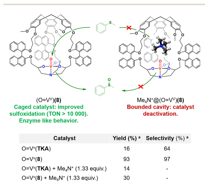
Fig. 8 (Top) Representation of the efficient sulfidation observed in caged oxido-vanadium catalyst ( O=V^V(\mathbf{8}) ) (left), and catalyst inhibition observed upon tetramethylammonium binding in the catalyst cavity (right). (Bottom) Comparison with its open analogue devoid of the CTV cap ( O=V^V(\mathbf{TKA}) ). a Oxidation of thioanisol in the presence of the catalyst (1.5 mol%) and CHP (1.0 equiv.) for 180 min in CH_2Cl_2 at 0 °C.
