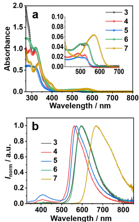
Fig. 2 (a) UV-vis absorption spectra and (b) emission spectra ( \lambda_{\text{ex}} = 320 \text{ nm} ) of 3–7 in CH 2 Cl 2 (1.0 × 10 -5 mol L -1 ).
