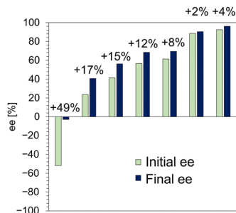
Fig. 5 Enantio-enrichment of 1 by enantioselective dissolution in methanol.
