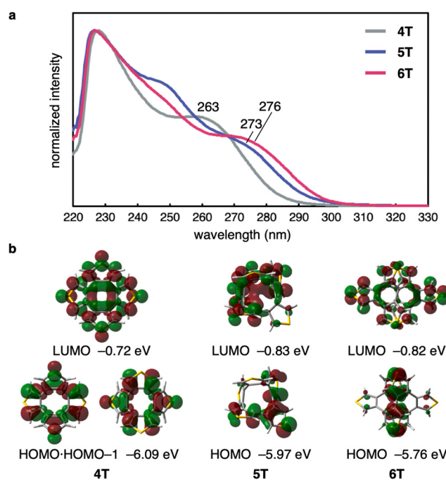
Fig. 5 Optoelectronic properties of 4T, 5T, and 6T. (a) UV-vis absorption spectra of 4T, 5T, and 6T in \text{CH}_2\text{Cl}_2 . (b) Frontier molecular orbitals and the energy levels of 4T, 5T, and 6T calculated at the B3LYP-D3/6-31G(d) level (isovalue = 0.03).
