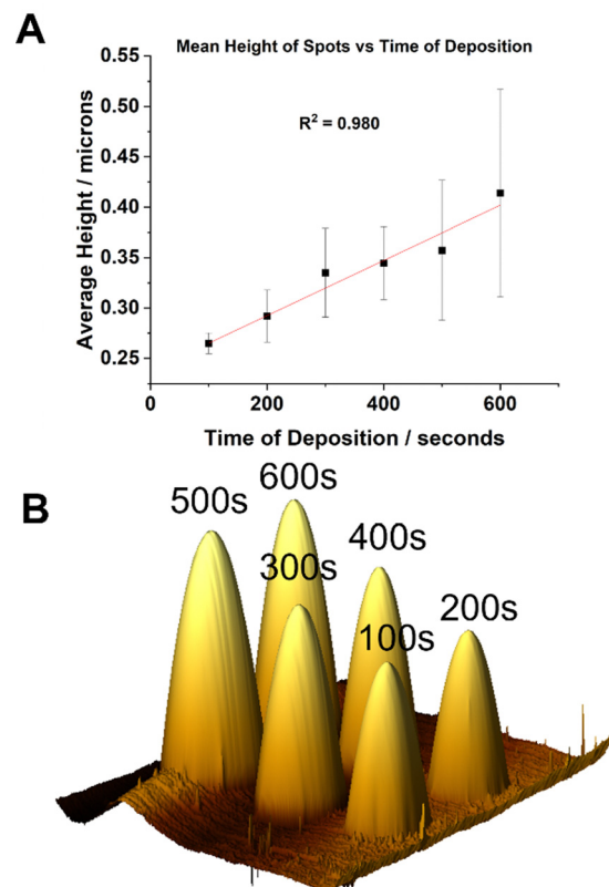
Fig. 4 Si-eATRP of Am at a SAM-functionalised gold electrode using [Am] = 10 wt% and [ \text{Cu}^{\text{II}} ]/[TPMA] = 6.9 mM; (A) feature height as function of reaction time; (B) 3D representation of the AFM image of features deposited at E_{\text{app}} = -0.15 V at increasing reaction times (100–600 s).
