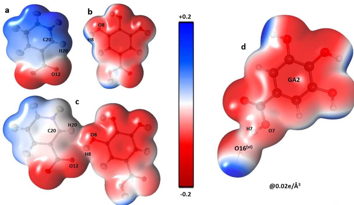
Fig. 6 The three-dimensional electron density of NA1 (a), GA2 (b), the co-crystal NA1-GA2 dimer (c) and \text{GA2} \cdots \text{O16}^{\text{vi}} (d); symmetry code the same as mentioned in Table 2, generated at isosurface value of 0.02 \text{ e } \text{Å}^{-3} coloured according to electrostatic potential using experimental data.
