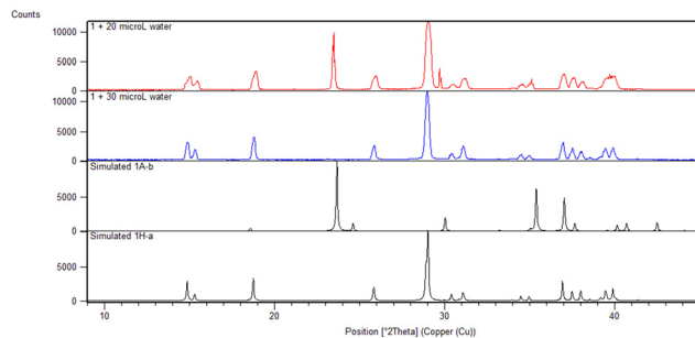
Fig. 1 PXRD pattern of 1 sublimed with 20 \mu\text{L} water (red) and 30 \mu\text{L} water (blue), compared to simulated patterns (black) for the anhydrous and hydrate crystals.
