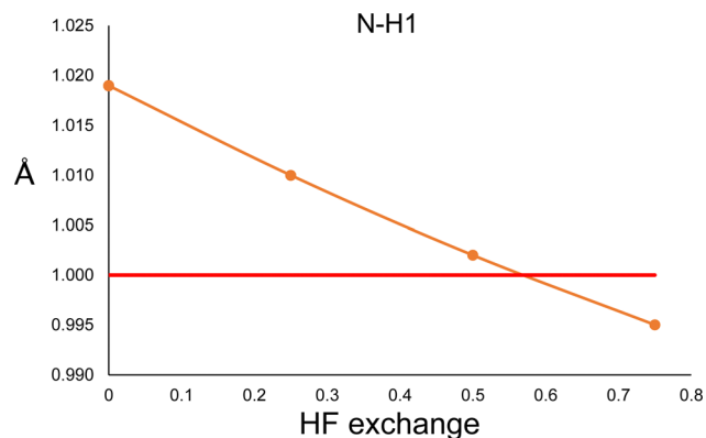
Fig. 4 N–H1 distance obtained from a constrained geometry optimisation with periodical DFT calculations, performed with the PBE functional and different amounts of Hartree–Fock exchange. The red line corresponds to the neutron diffraction value.
