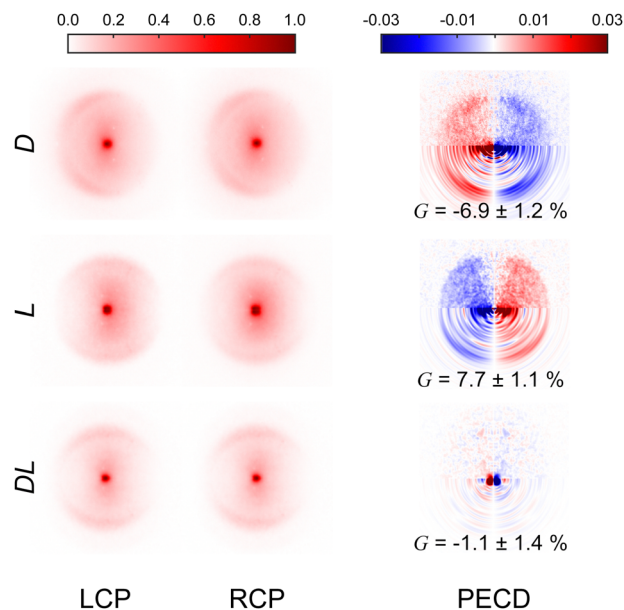
Fig. 3 Experimental VMI images recorded for D-, L- and DL-phenylalanine using both LCP and RCP. The laser propagation direction is from left to right and the images are 2-fold symmetrized ( i.e. the top and bottom halves of the raw data have been averaged together – which is valid given the symmetry of the photoelectron angular distribution described by eqn (2)). The PECD difference images (LCP – RCP) are also included in the right-hand column. The lower half of these PECD images show processed output following application of the pBASEX method. A clear asymmetry is present in the PECD images for each enantiomer. For D-phenylalanine, the PECD image reveals an overabundance of photoelectrons detected in the backwards direction (indicated by red on the colour scheme) with a corresponding depletion of electrons in the forwards direction (blue). This asymmetry is of similar magnitude for L-phenylalanine, but of opposite sign (red and blue are exchanged). Within a small degree of background noise, no significant asymmetry is seen for racemic phenylalanine, as expected. See text for details and discussion.
