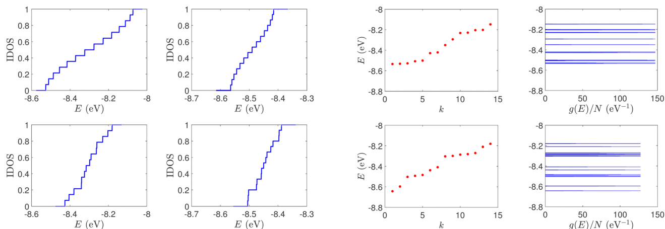
Fig. 2 Normalized IDOS of the unmutated DNA sequences depicted in Fig. 1. Upper panels: Ideal, lower panels: natural, left panels: G_{14} , right panels: A_{15} .
