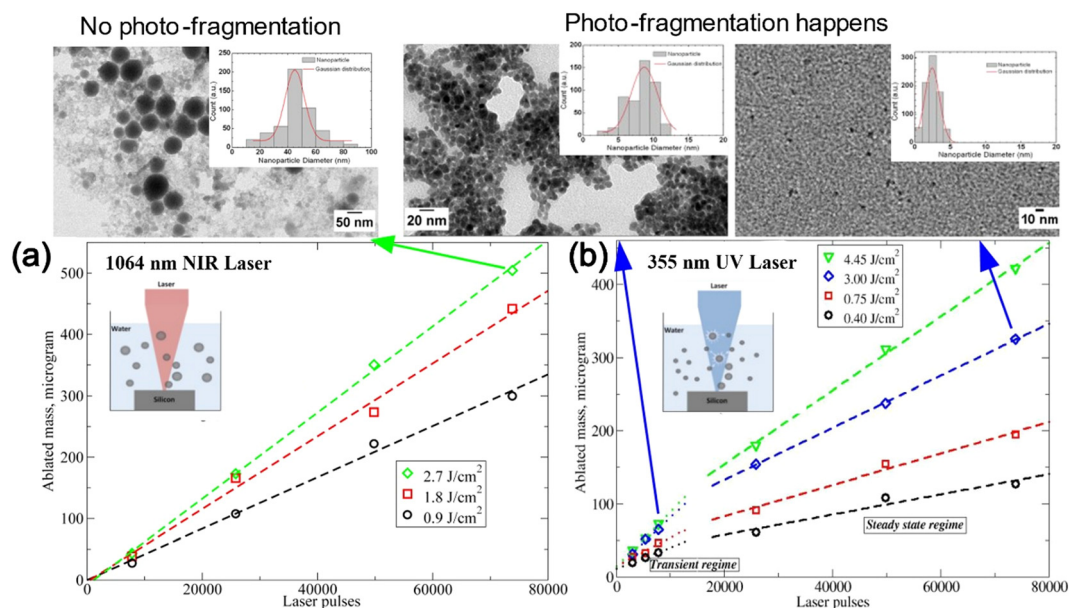
Fig. 7 Laser wavelength influence on the productivity and particle size of Si ablation in water. (a) Ablation using a 1064 nm NIR laser shows steady mass as a function of a number of pulses (ablation time) in different fluences. The inset, indicated by the green arrow, shows the TEM image and particle size distribution of Si ablated using a 1064 nm NIR laser. (b) Ablation using a 355 nm UV laser produces smaller Si NPs with increasing ablation time due to photo-fragmentation. Insets, indicated by the blue arrows of the respective data point, show the TEM image and particle size distribution of Si ablated using a 355 nm UV laser. Adapted from ref. 131 with permission from The Optical Society, copyright 2014.
