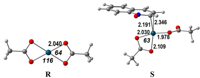
Scheme 5 The geometries of Pd(OAc) 2 (left panel) and [Pd(OAc) 2 (η 2 -QO)] (right panel).
