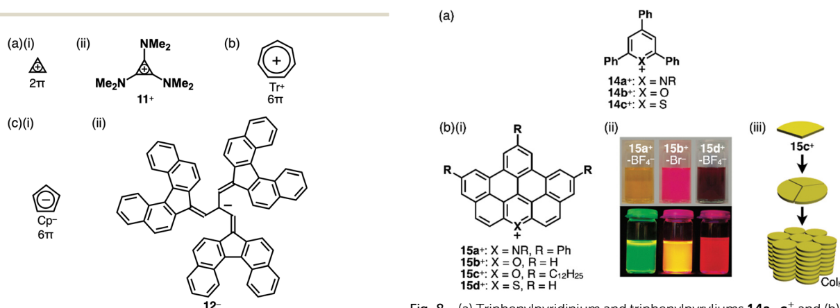
Fig. 6 Representative charged \pi -electronic systems stabilized by aromaticity: (a) (i) cyclopropenium and (ii) tris(dimethylamino)-substituted derivative 11^+ , (b) tropylium and (c) (i) cyclopentadienide and (ii) Kuhn's anion 12^- .
