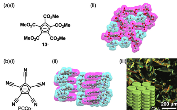
Fig. 7 (a) (i) Pentamethoxycarbonylcyclopentadienide 13^- and (ii) single-crystal X-ray structure of TMA^+-13^- and (b) (i) pentacyanocyclopentadienide ( PCCp^- ), (ii) single-crystal X-ray structure of (C_4H_9)(CH_3)_3N^+-PCCp^- and (iii) POM of liquid crystal mesophase of (C_{12}H_{25})_3CH_3N^+-PCCp^- at 70^\circ C upon cooling (redrawn from ref. 33. Copyright 2016 Wiley). The crystal structures are redrawn from cif files: 1137646 and 1431736.
