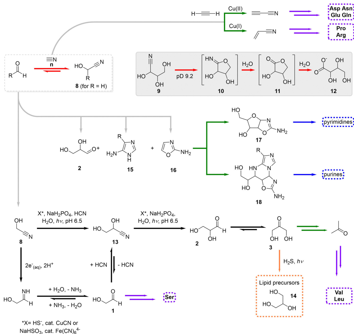
Scheme 7 Schematic overview of the cyanosulfidic scenario, highlighting its initiation through glyconitrile formation and associated reactions (red transformations), the core homology steps of this scenario (black), and the most important routes towards purine and pyrimidine ribonucleotides (blue), lipid precursors (orange), amino acids (purple) and other key intermediates (green). 14,20,99 Only the key intermediate compounds have been numbered.
