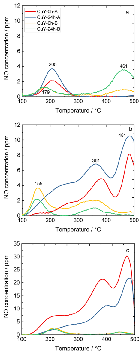
Fig. 8 TPD-NO x profiles of copper-containing zeolite Y samples: a) NO x desorption in He (pre-treatment in He), b) NO x desorption in a 4 vol% O 2 /He mixture (pre-treatment in He), and c) NO x desorption in He (pre-treatment in 5 vol% O 2 /He); the sample labels are the same for a)-c).
