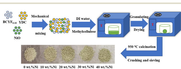
Fig. 1 Schematic diagram of the catalyst particle preparation process.
