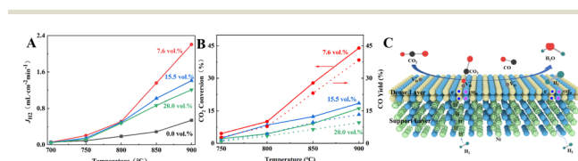
Fig. 7 (A) H 2 permeation flux, (B) CO 2 conversion and CO yield as a function of temperature for BCYF 0.10 -YDC/BCYF 0.10 -Ni dual-layer HF membranes under different concentrations of CO 2 sweeping (feed gas was 100 mL min -1 of 50 vol% H 2 /He mixture and sweep gas was 100 mL min -1 of N 2 with different concentrations of CO 2 ); (C) schematic illustration of H 2 permeation through dual-layer HF membranes under CO 2 sweeping conditions.
