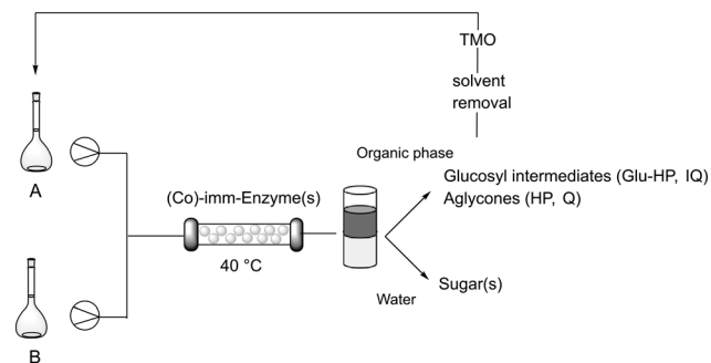
Scheme 2 Flow bioprocessing of HES and RT. Solution A: 10 g\ L^{-1} HES or RT in TMO. Solution B: HEPES buffer, 0.05 M, pH 7.5. Co-imm-enzyme(s): imm-RN (5 mg g_{\text{resin}}^{-1} ) or HOR (1 mg g_{\text{resin}}^{-1} ) or imm-RN-HOR (5 mg RN g_{\text{resin}}^{-1} , 1 mg HOR g_{\text{resin}}^{-1} ). T = 40\ ^\circ\text{C} .
