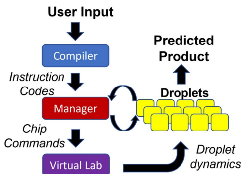
Fig. 10 Block diagram of the software modules that plan and execute the automated gene assembly. The Compiler reads the desired input and consults a preprogrammed chemical protocol to generate the necessary chemical operations and properly order them. The Manager reads the resulting instruction codes and coordinates the creation, destination selection, and routing of droplets. The Virtual Lab provides feedback on droplet movements to the manager.
