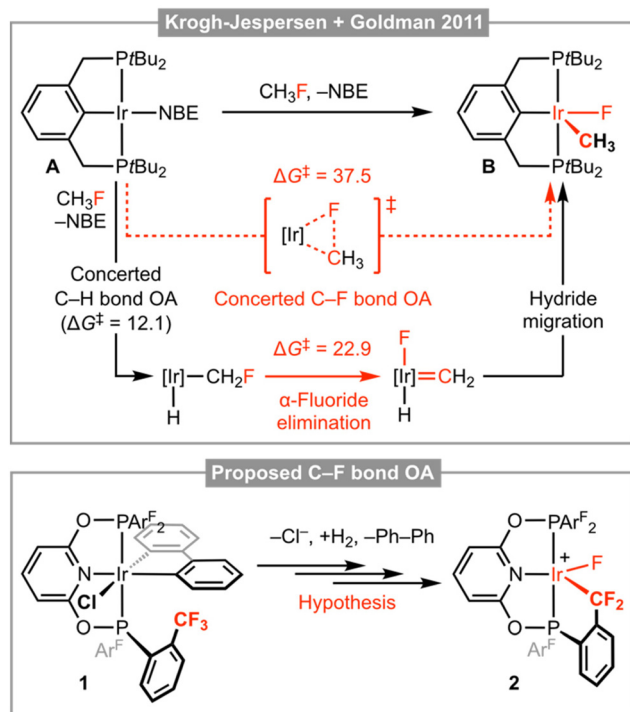
Fig. 1 Activation of fluoromethane by an Ir(PCP) pincer complex and proposed intramolecular C(sp 3 )-F bond activation manifold. Calculated activation barriers in kcal mol -1 relative to A; NBE = norbornene.
