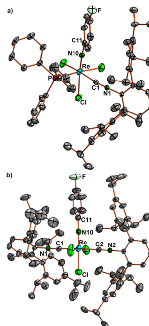
Fig. 5 Molecular structures of (a) fac- [\text{Re}(\text{NPhF})\text{Cl}_3(\text{PPh}_3)(\text{CNAr}^{\text{Tripp}2})] ( 9 ) and (b) mer- [\text{Re}(\text{NPhF})\text{Cl}_3(\text{CNAr}^{\text{Tripp}2})_2] ( 10 ). Selected bond lengths and angles of 9 : Re–N10 1.711(4), Re–P 2.460(2), Re–C1 2.027(5), C1–N1 1.167(5) Å; Re–N10–C11 168.7(3), and Re–C1–N1 170.4(4)°. Selected bond lengths and angles of 10 : Re–N10 1.698(6) and 1.711(5), Re–C1 2.093(6) and 2.090(6), Re–C2 2.084(6) and 2.076(6), C1–N1 1.135(7) and 1.139(7), C2–N2 1.135(7) and 1.148(7) Å; Re–N10–C11 177.1(5) and 178.7(5), Re–C1–N1 175.3(6) and 178.2(6), and Re–C2–N2 175.4(5) and 179.5(7)°. The values of compound 10 refer to two independent molecular species.
