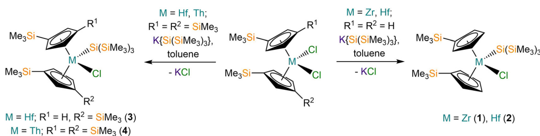
Scheme 1 Synthesis of 1–4.
