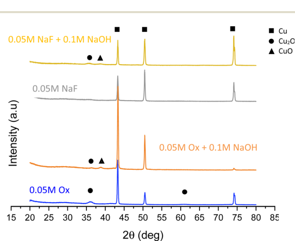
Fig. 5 XRD patterns of copper oxide nanostructures after anodization at 20 V and 50 °C in different electrolytes with 70% (v/v) EG and at 0 rpm.
