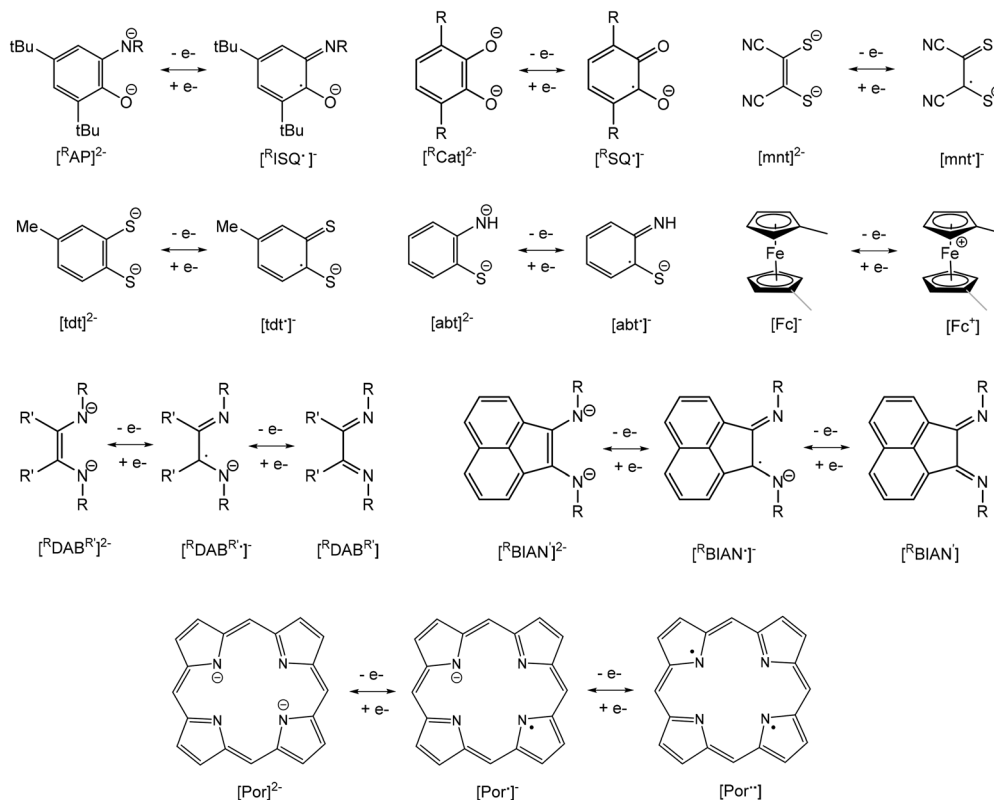
Fig. 1 Redox couples of redox-active ligands capable of acting as electron reservoirs: o -amidophenolate (AP)/ o -iminosemiquinone (ISQ), catecholates (Cat)/ o -semiquinone (SQ), maleonitriledithiolate (mnt), 3,4-toluenedithiolate (tdt), 2-amidobenzenethiolate (abt), ferrocenyl (Fc), 1,4-diaza-1,3-butadiene (DAB), 1,2-bis(imino)acenaphthene (BIAN) and porphyrinato (Por).
