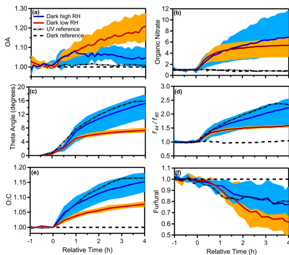
Fig. 6 Enhancement (normalized to initial values of 1) in (a) OA, (b) organic nitrate, (c) change in theta angle in degrees, (d) f_{44}/f_{60} , (e) O : C ratio, and (f) fural ( m/z 97) for the dark aging experiments under dry (experiments 1 to 3) and high RH (experiments 4 to 6) conditions. The shaded blue (dark RH experiments) and orange (dark dry experiments) regions correspond to the variability across all experiments due to differences in injected \text{NO}_2 and \text{O}_3 concentrations, while the solid blue and red lines are the median across the RH and dry experiments, respectively, and the dashed black lines correspond to UV (experiment 7) and dark reference (experiment 8) experiments.
