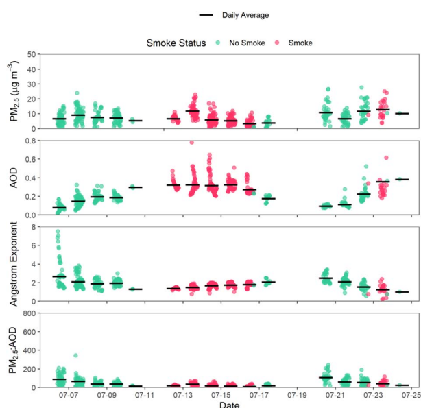
Fig. 6 Time-series plots of \text{PM}_{2.5} , AOD, Angstrom exponent, and \text{PM}_{2.5}:\text{AOD} ratio from July 6, 2021, to July 24, 2021, from four CEAMS sites in Southern California, colored by HMS-derived smoke status. Measurements are from four AMODv2s (Fig. 1). Note that measurements on July 12, 2021, were from a single AMODv2 started early by the CEAMS participant.
