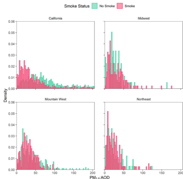
Fig. 7 Regional density histograms for \text{PM}_{2.5}:\text{AOD} ratio separated by HMS smoke status. Note that here we refer to the "California/West Coast" region as "California" because sites in Washington and Oregon did not collect valid AOD measurements.
