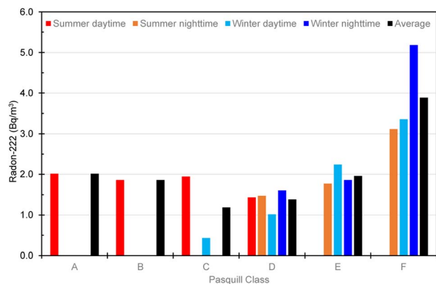
Fig. 4 Radon-222 activity concentration ( \text{Bq m}^{-3} ) in the surface air classified according to modified Pasquill stability class, Sevettijärvi, northern Finland.
